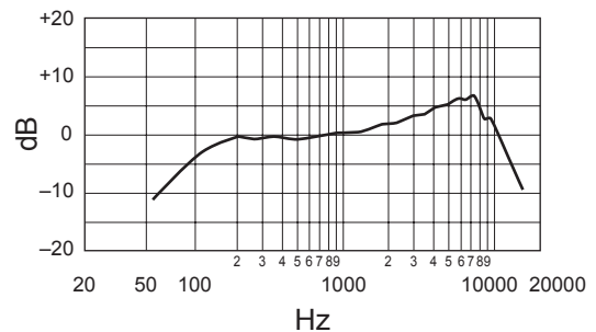
Frequency Response
