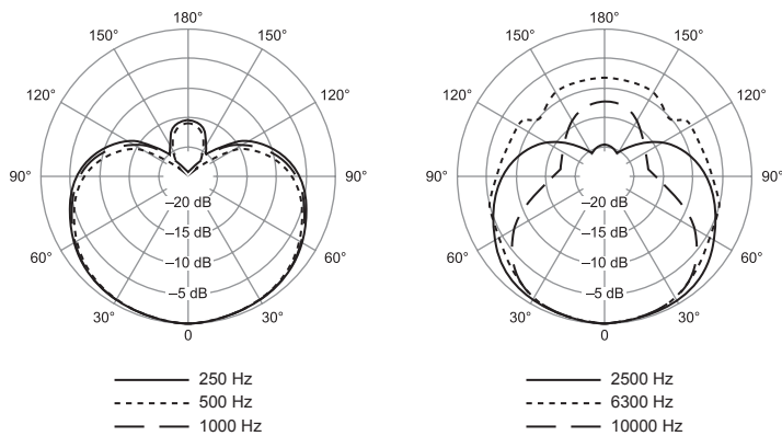
Polar Pattern Measured at 1000 Hz
