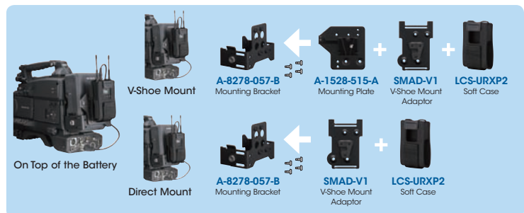
SMAD-V1 V-Shoe Mount Adaptor for LCS-URXP2
