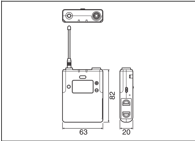
63 × 82 × 20 mm (2 1/2 × 3 1/4 × 13/16 in.) (Width / height / depth) (excluding antenna)
