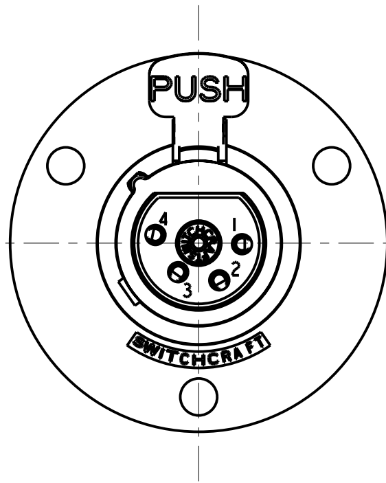
4 PIN
