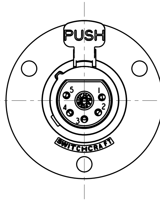
6 PIN
