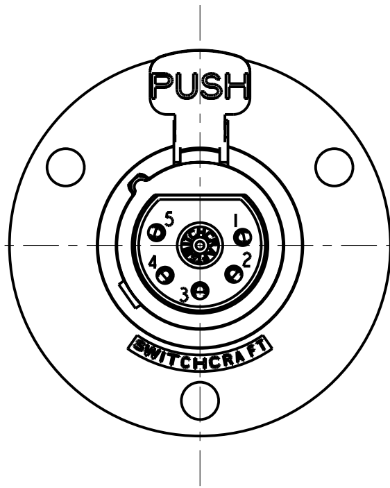
5 PIN
