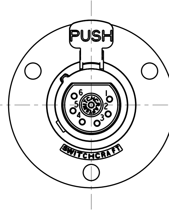
7 PIN
