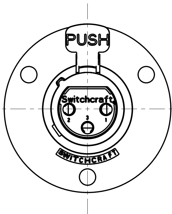
3 PIN
