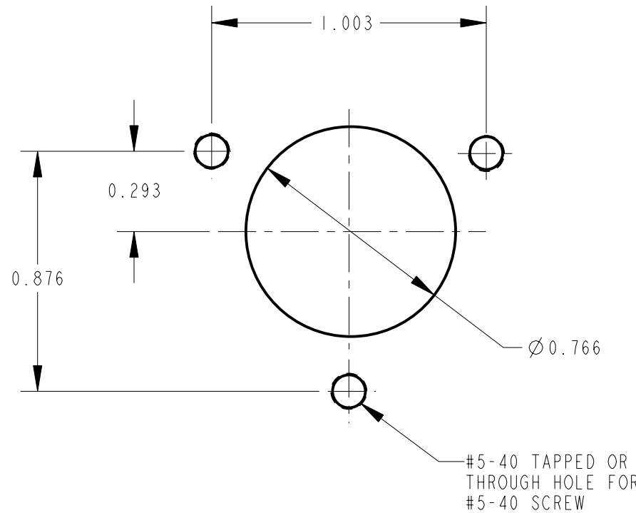
RECOMMENDED PANEL CUT-OUT
