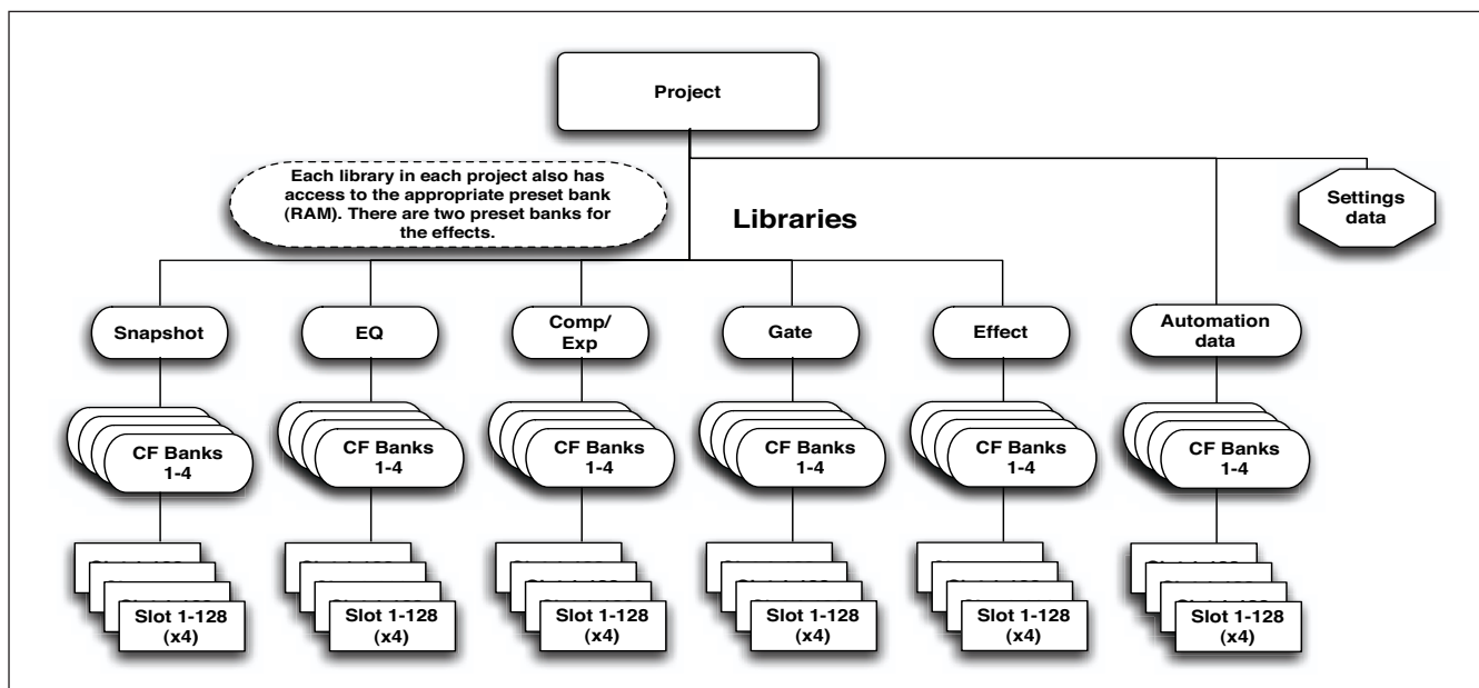
Figure 2.29: Project structure
