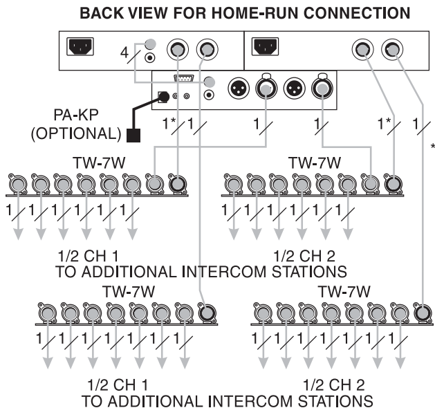
Figure 7. US2002 Monaural Master Speaker Station Configuration with 2 Power Supplies. This is a good configuration for large intercom systems when you want to operate the US2002 as a master speaker station, with one speaker to monitor both intercom channels. In this configuration, the SPS2001 and PS2001L Combine/Isolate switches are set to the Combine position. With this setting all intercom stations connected to the SPS2001 are combined on intercom channel 1 and all intercom stations connected to the PS2001L are combined on channel 2. The amplified speaker in the SPS2001 is used as the speaker output for the US2002 and the US2002 dip switches are set to monaural operation (default setting) so that both intercom channels are heard in the speaker. The PA-KP local power supply is optional. When a PA-KP is connected, the US2002 automatically disconnects from system power. Since the US2002 is not drawing power from the intercom system, more system power is available for additional belt packs, etc.
