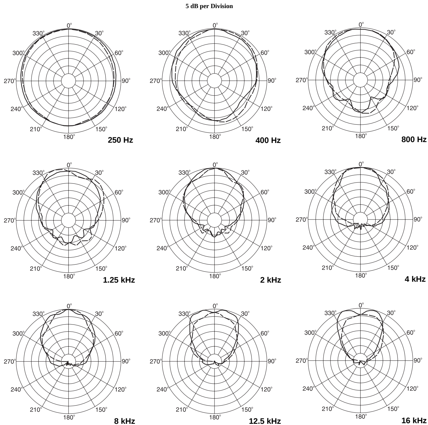
Figure 2 — Sx300 Polar Response (anechoic environment)
