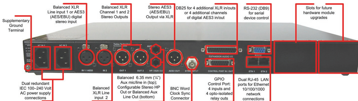
Merlin rear panel
