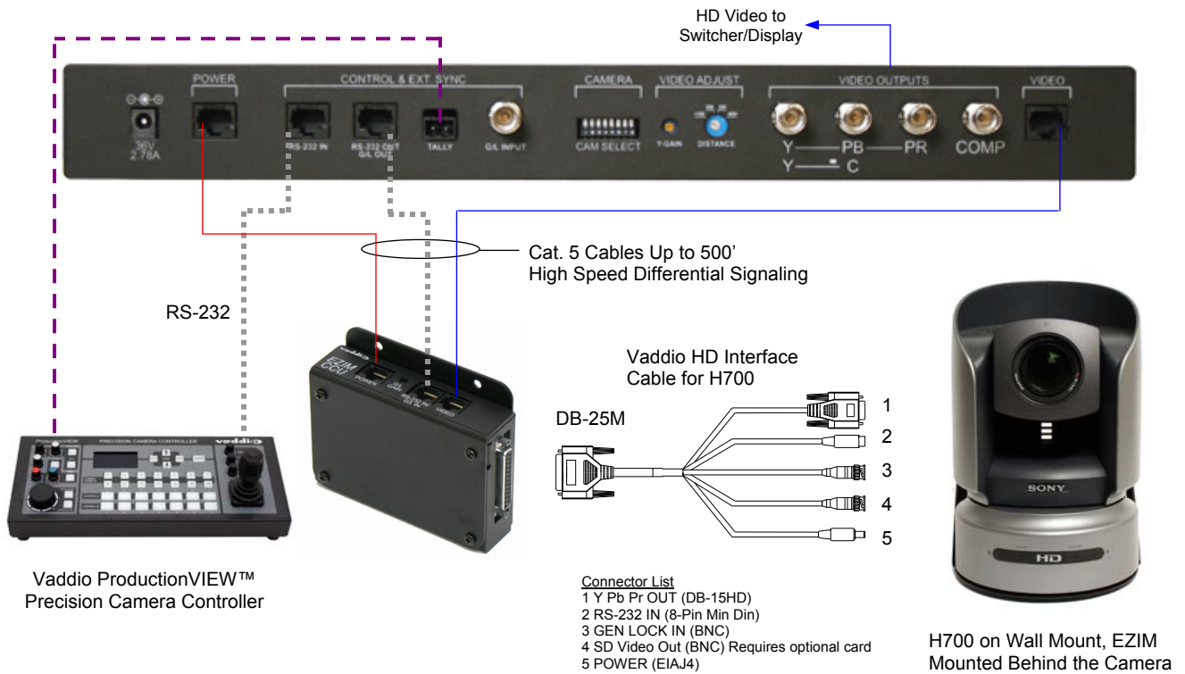
Figure 4: Basic system connectivity of a WallVIEW CCU H700 System and ProductionVIEW Precision Camera Controller
