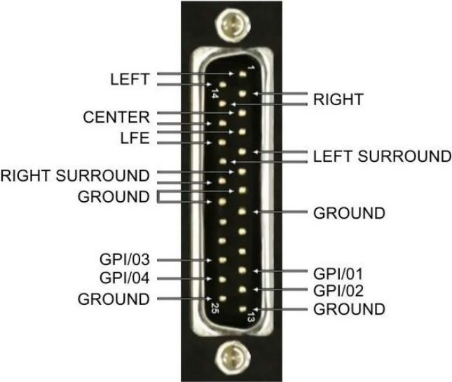
AUX 2 ANALOG AUDIO OUTPUT
