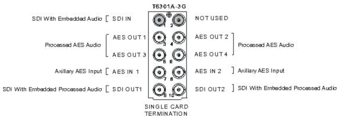
Figure 2. Rear Modules
