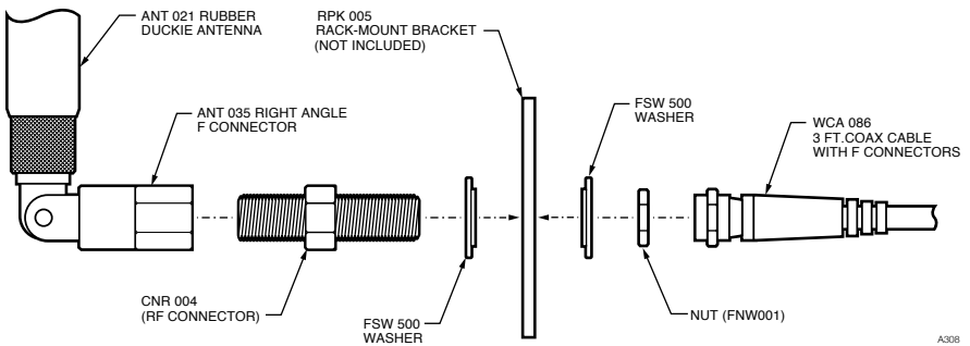
Figure 1: ANT 034 Assembly
