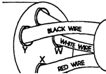
CONNECTOR WIRING DETAIL
