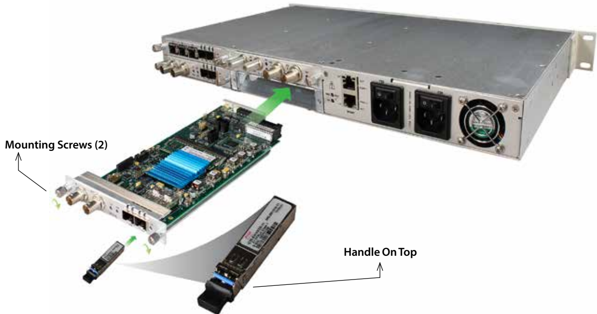
Figure 4. ILC450 Module and SFP+ Installation
