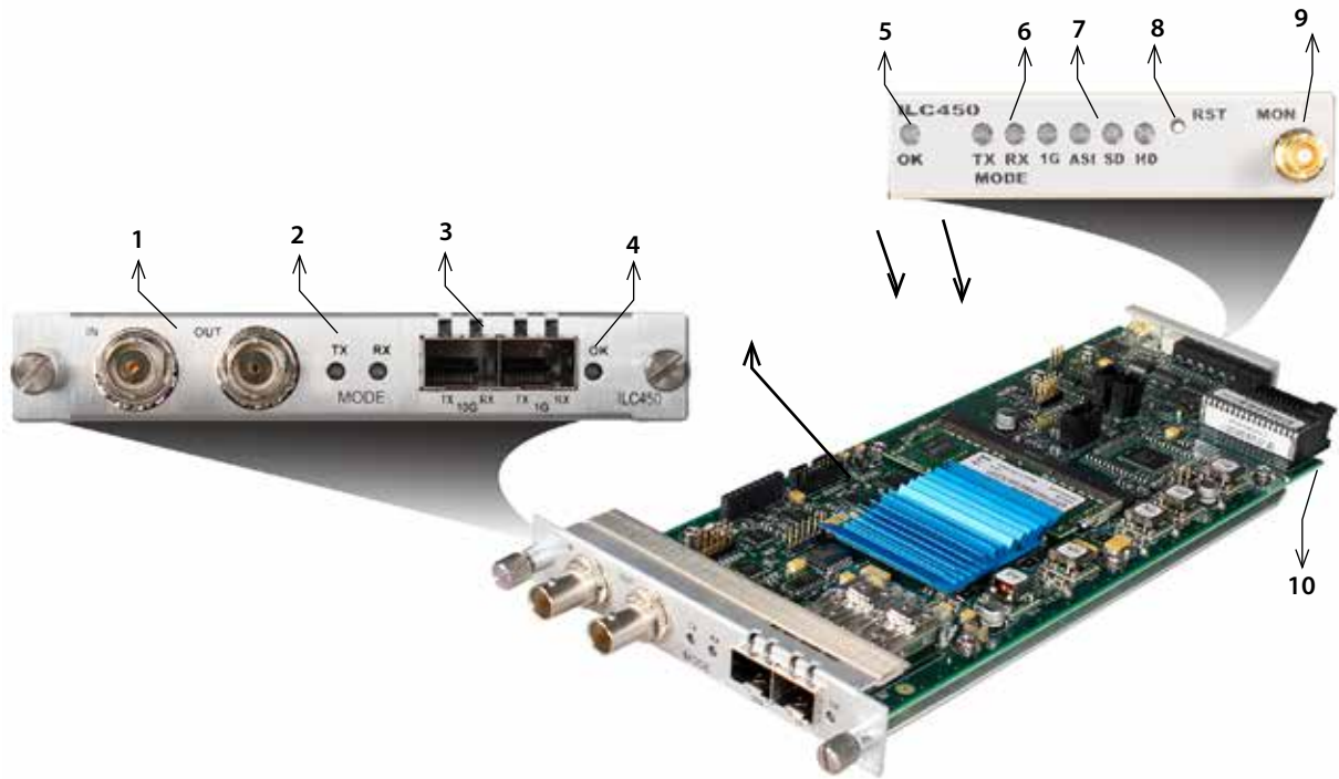
Figure 3. ILC450 Module Major Components
