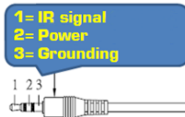
IR Receiver
