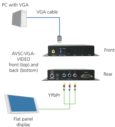
Figure 3-1. Typical application.
