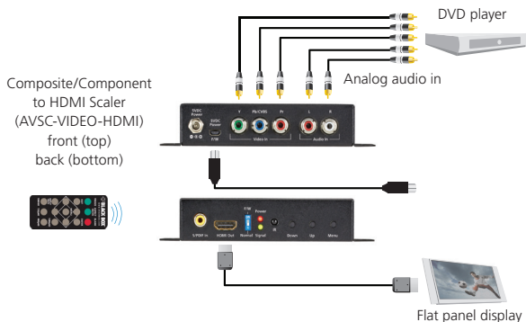
Figure 3-1. Typical application.
