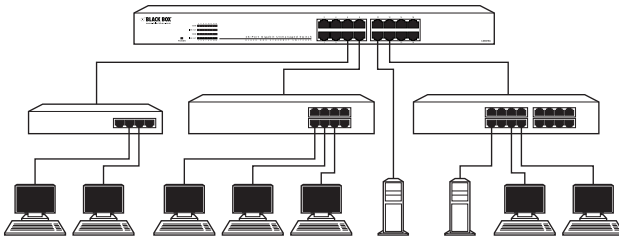
Figure 3-1. Switch/hub connection.
