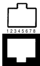
RJ45 SOCKET/PLUG PIN DIAGRAM
