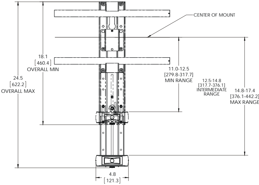
FUSION WALL BELOW MOUNT SETUP
