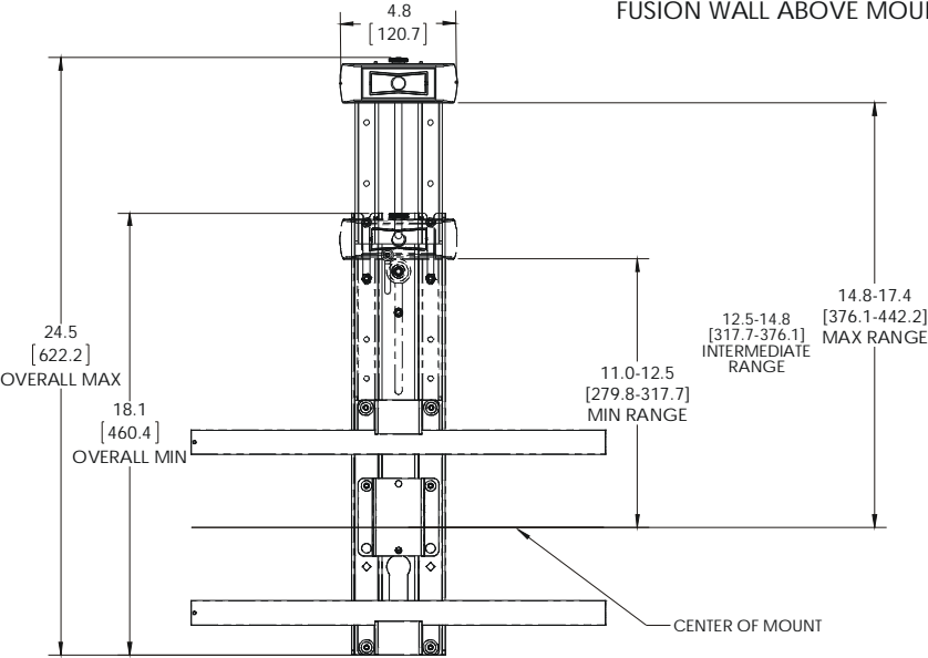
FUSION WALL ABOVE MOUNT SETUP
