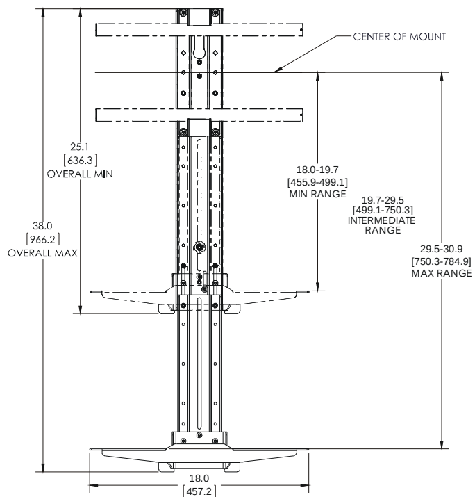
FUSION CEILING BELOW MOUNT SETUP
