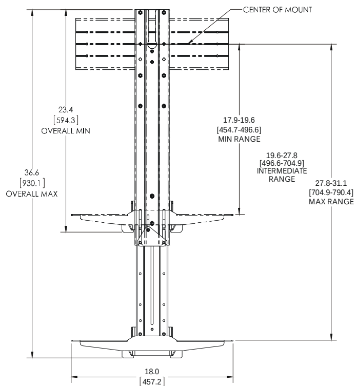
FUSION CEILING BELOW MOUNT SETUP
