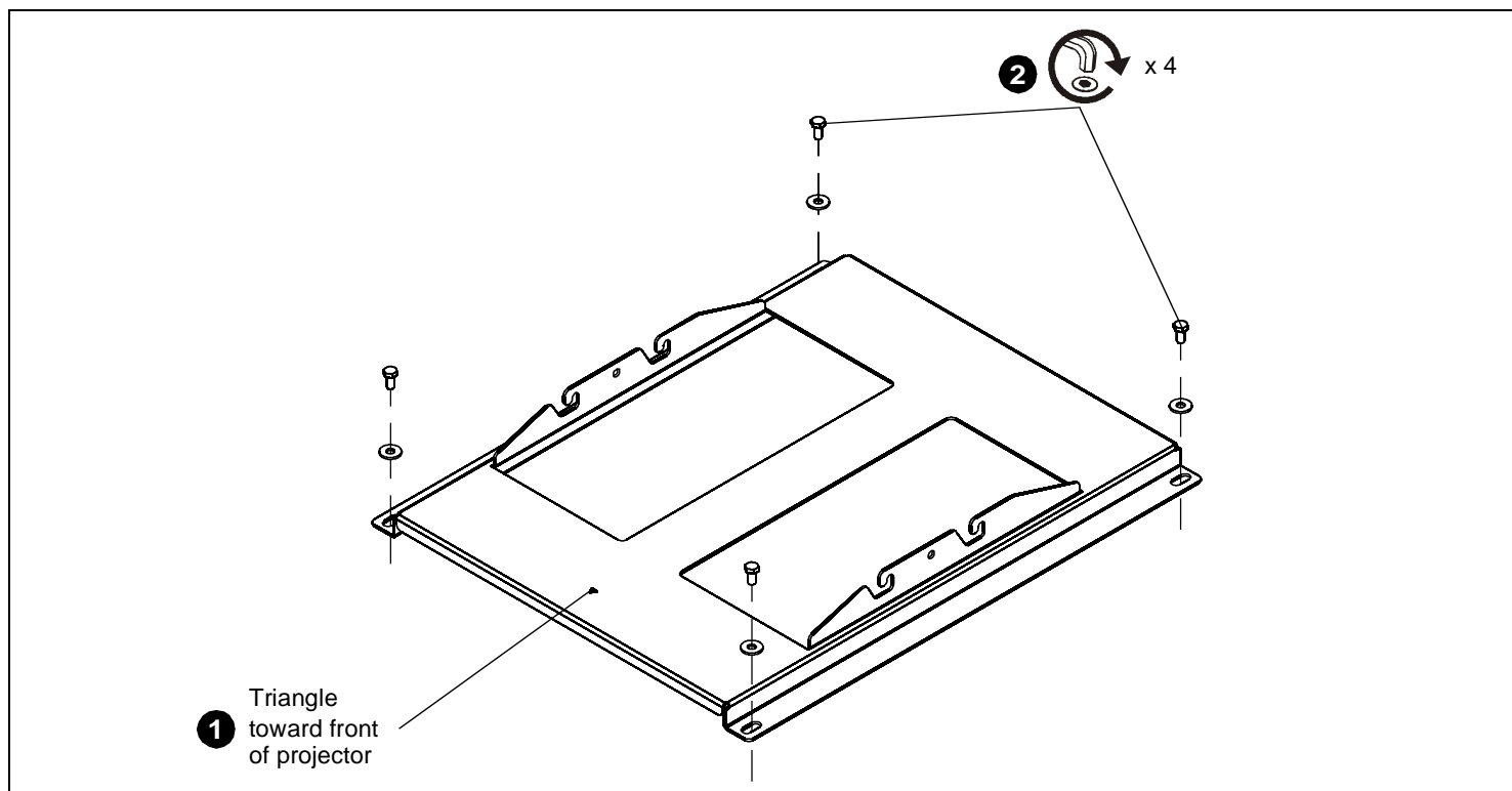
Figure 1: INSTALLATION
