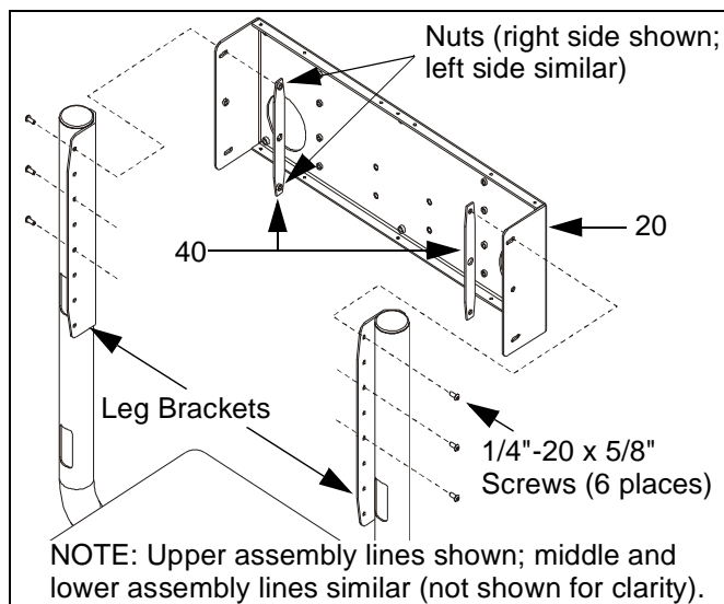
Figure 4: Install Dual Mount Head
