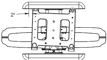
Roll Adjustment
