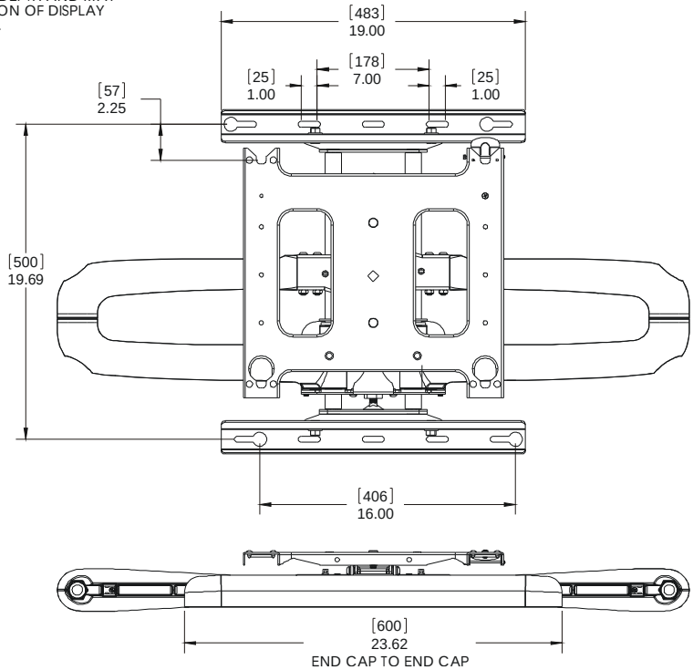
Mounting Pattern
