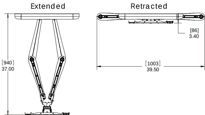
Unit Depth
