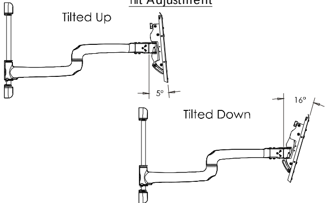
Tilt Adjustment *
