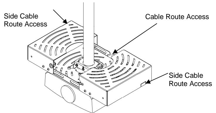
Figure 5. Route Cables
