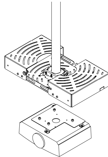
Figure 4. Install Projector
