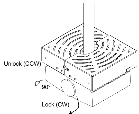
Figure 6. Lock Unit
