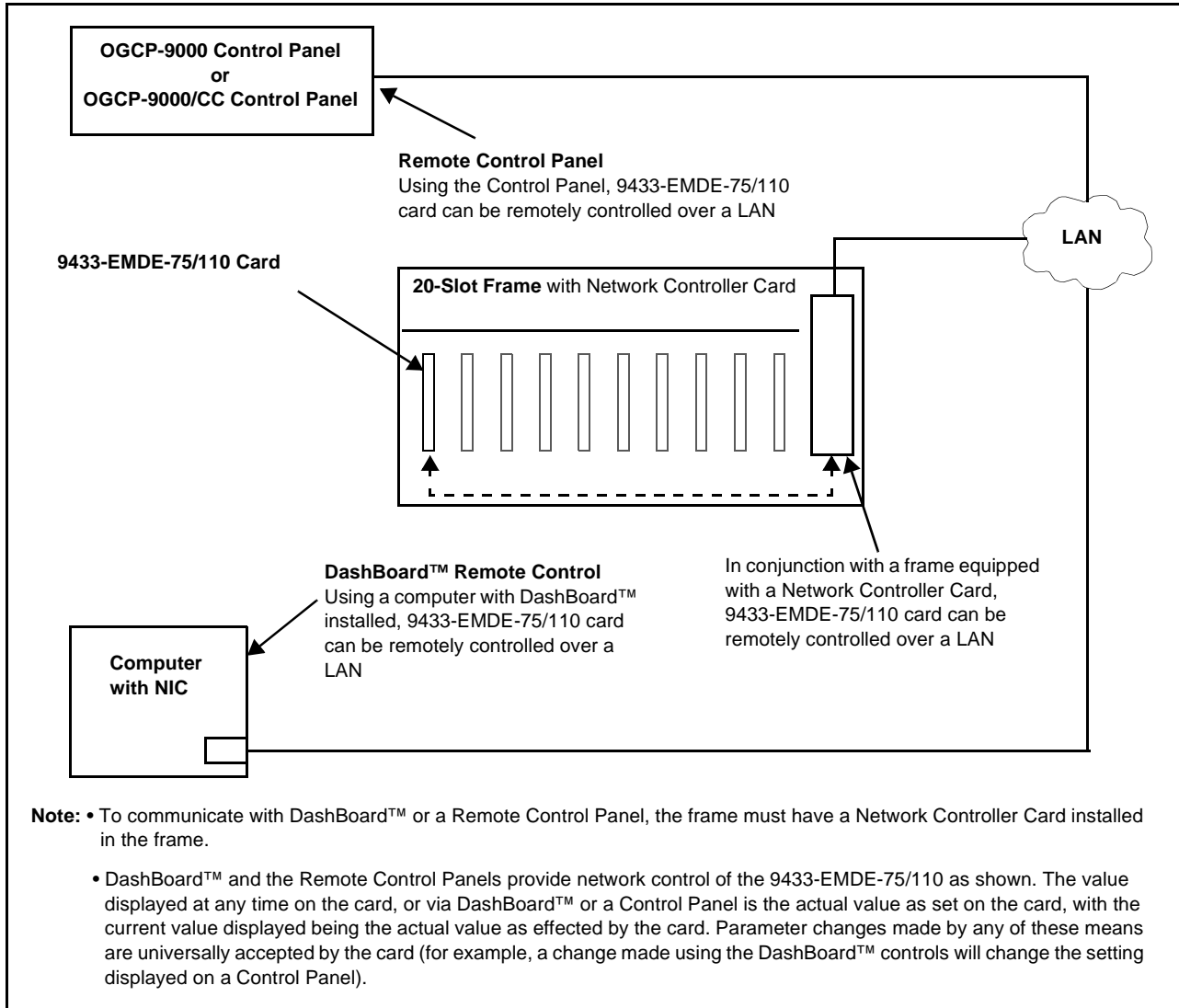
Figure 1-2 9433-EMDE-75/110 User Control Interface
