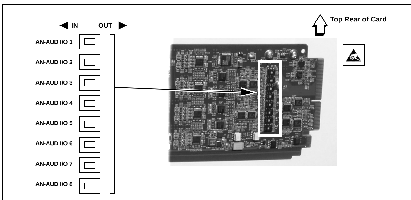
Figure 2-1 AN-AUD I/O (1-8) Direction Switches
