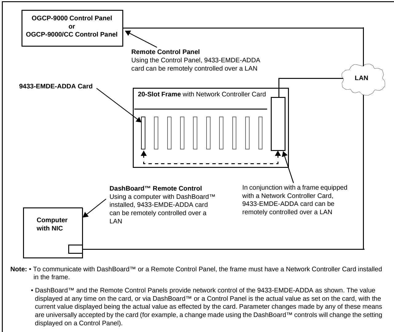
Figure 1-2 9433-EMDE-ADDA User Control Interface
