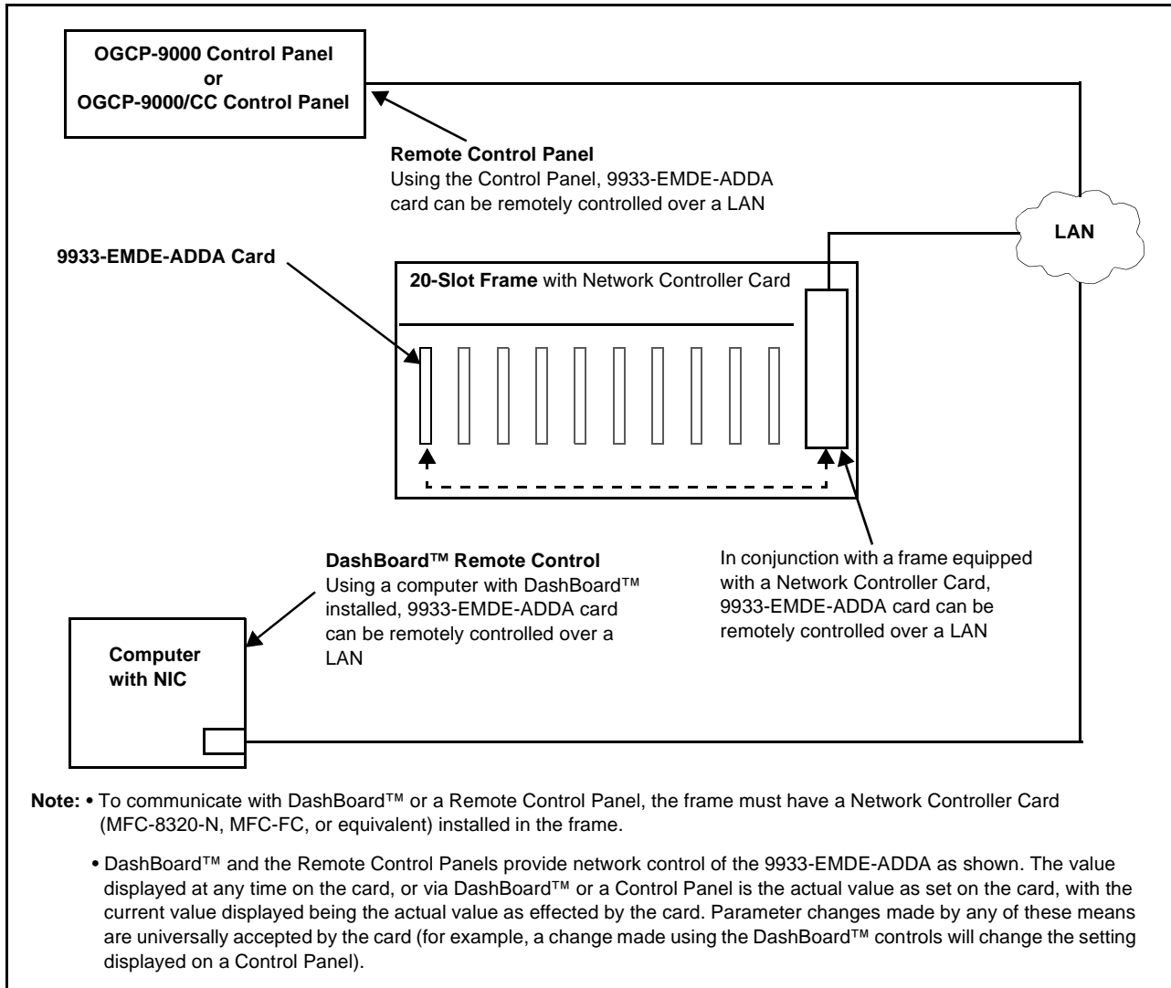
Figure 1-2 9933-EMDE-ADDA User Control Interface
