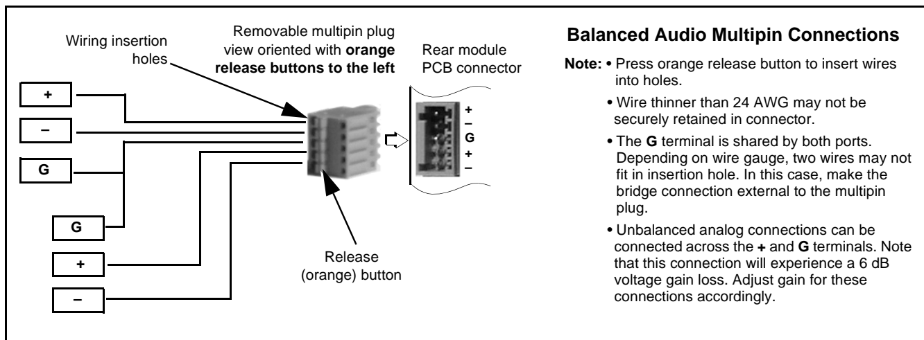
Figure 2-3 Balanced Audio Connections
