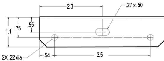
Mounting Flange Dimensions & Attachment Holes
