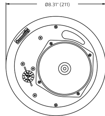
Figure 15. C4 loudspeaker dimensions
