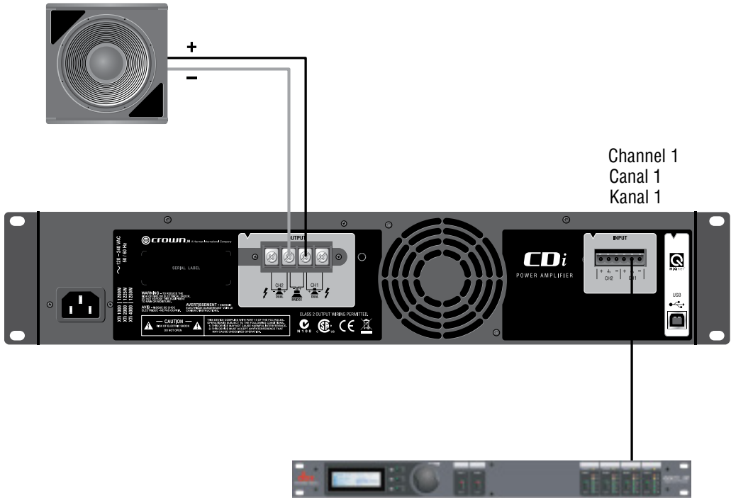
Figure 2.6 System Wiring, Bridge-Mono Mode
