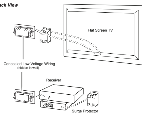
Figure 3 - Back View
