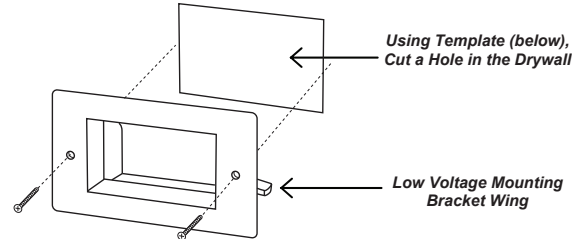
Figure 2 - Front View
