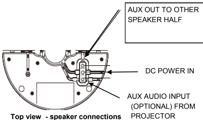
Top view - speaker connections on the powered half .
