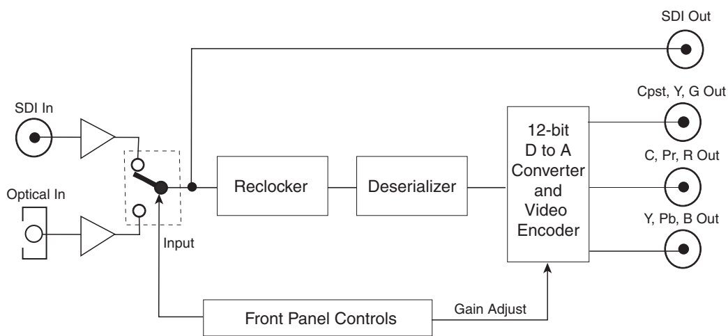
BrightEye 10 Functional Block Diagram
