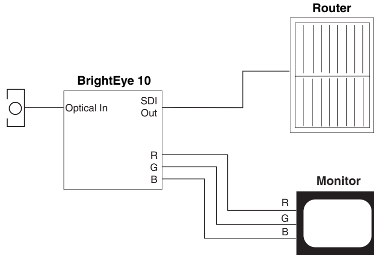
Optical to Electrical Conversion with Analog Monitoring Illustration
