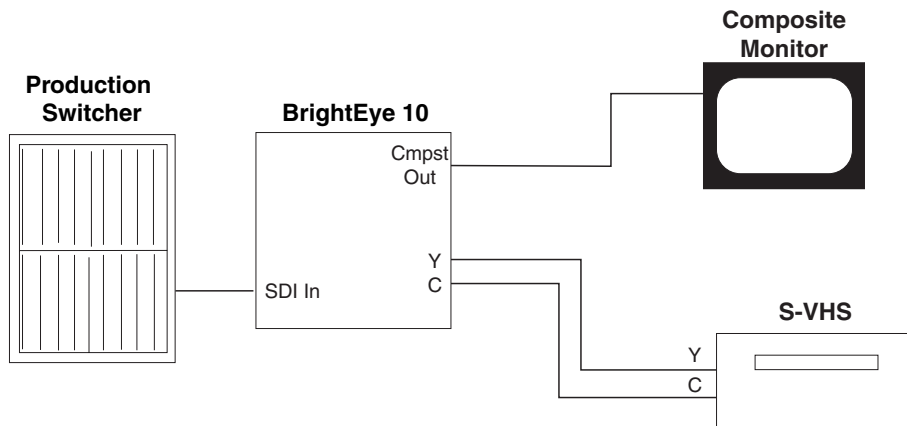
Analog Monitoring of an SDI Signal Illustration
