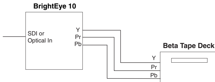
Optical or SDI Input to Component VTR Application
