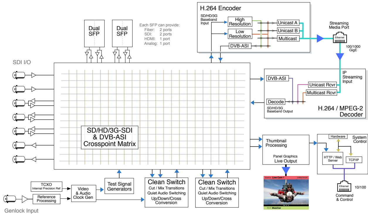
BrightEye NXT 450 Functional Block Diagram, Portrait View
