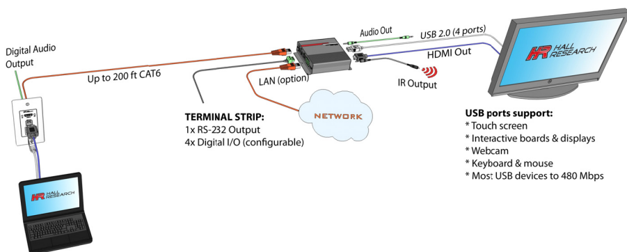
Typical Connection Diagram
