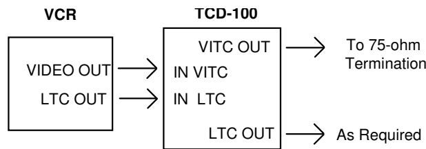
Figure 4-1, Basic TCD-100 Hookup
