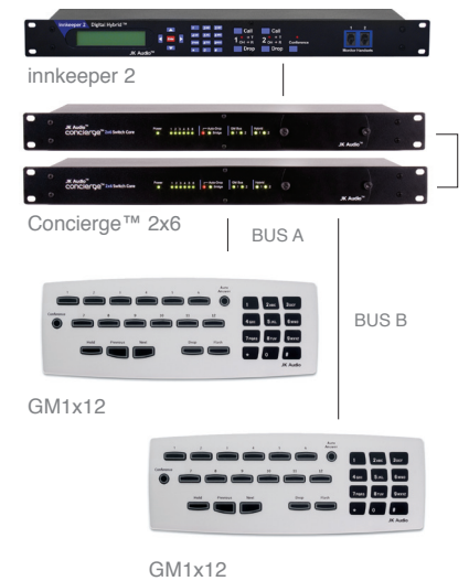
2 Hybrids, 12 Lines
