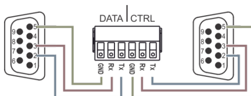
Figure 8: RS-232 Pinout
