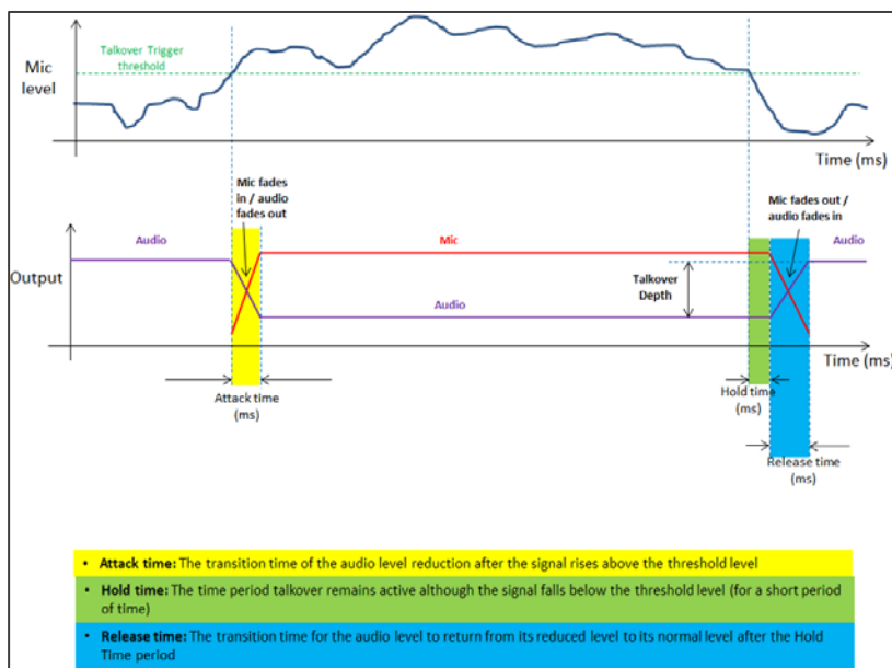
Figure 7: Talkover Mode
