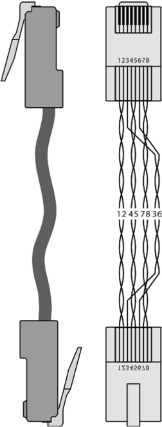
Figure 6: TP PINOUT
