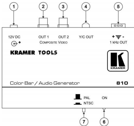
Figure 1: 810 Color Bar/Audio Generator
