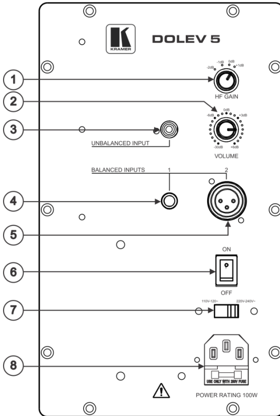
Figure 1: Dolev 5 Active 2-Way, Bi-Amplified Studio-Grade Speaker
