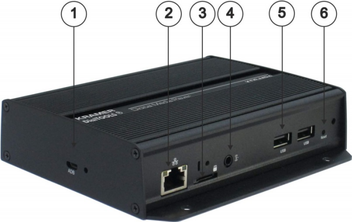
Figure 1: KDS-MP4 4K Digital Media Player - Front
