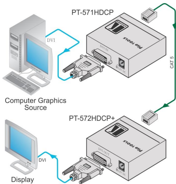
Figure 3: Connecting the PT-571HDCP/PT-572HDCP+ Transmitter/Receiver Pair
