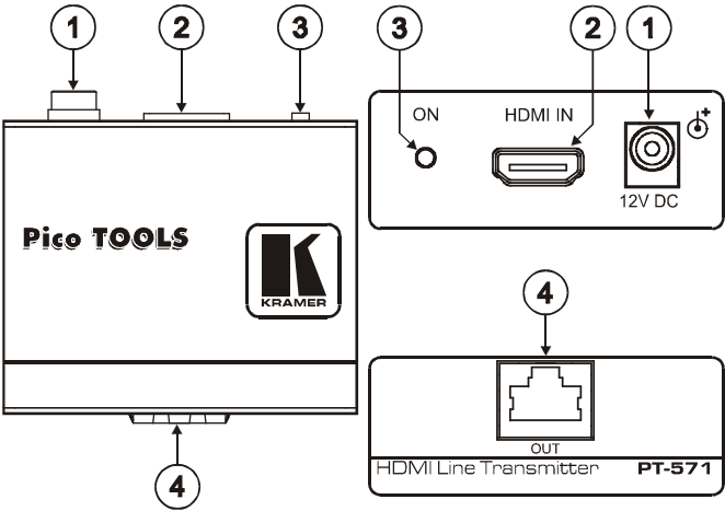
Figure 1: PT-571 HDMI Line Transmitter
