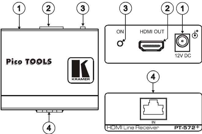
Figure 2: PT-572+ HDMI Line Receiver
