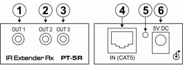
Figure 2: PT-5R IR Extender/Repeater
