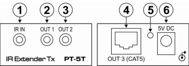
Figure 1: PT-5T IR Extender/Repeater
