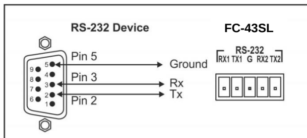
Figure 4: RS-232 Connection
