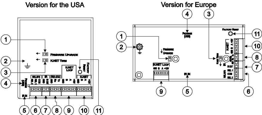
Figure 6: RC-63D Room Controller Rear Panel
