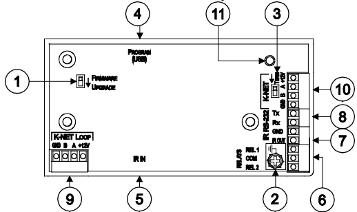
Figure 2: RC-62 Room Controller Rear Panel
