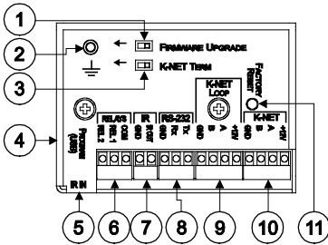
Figure 2: RC-62 Room Controller Rear Panel
