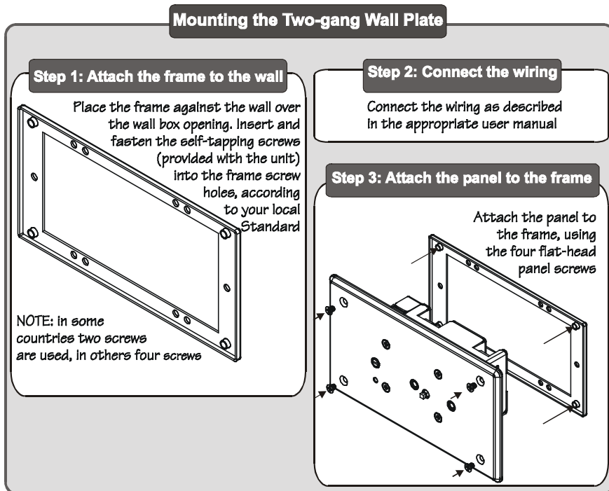
Figure 1: Mounting the Two-gang Wall Plate
