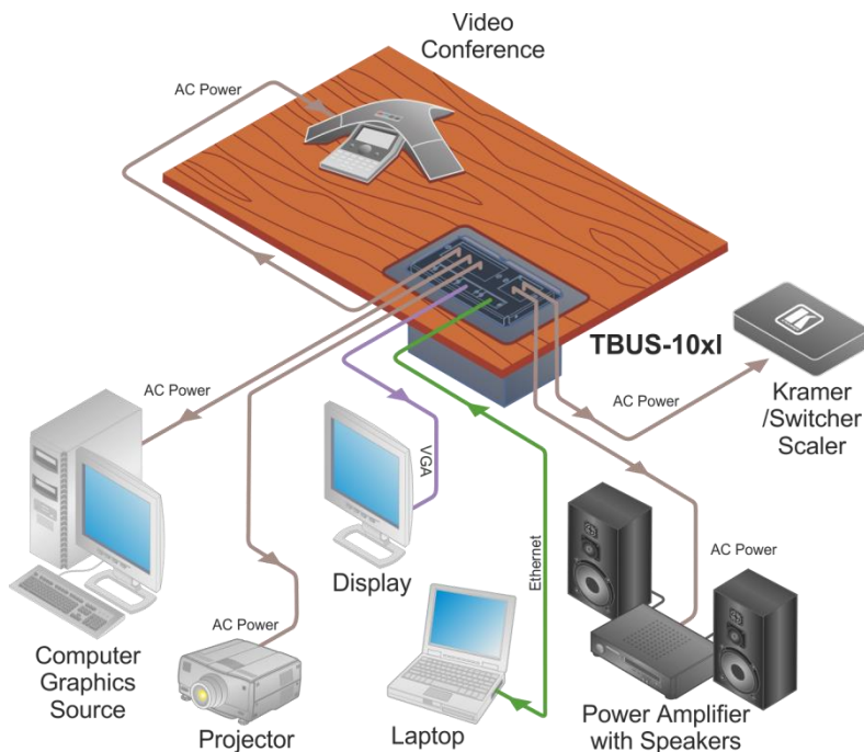
Figure 11: TBUS-10xl Boardroom Installation
