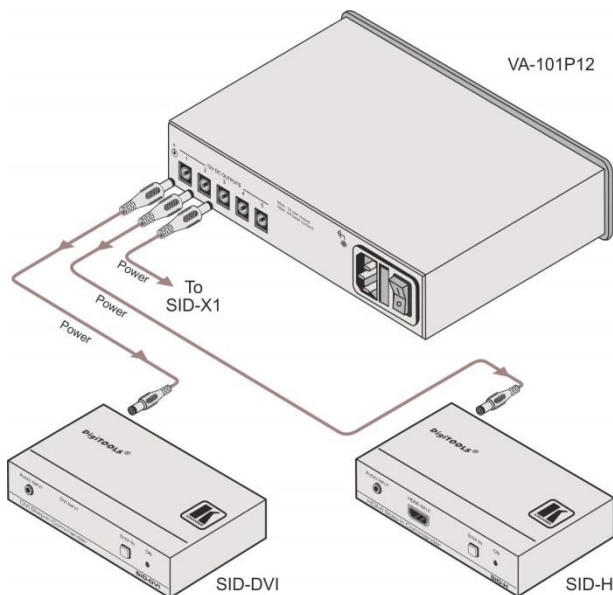
Figure 3: Connecting the VA-101P12, VA-102P12 Description
