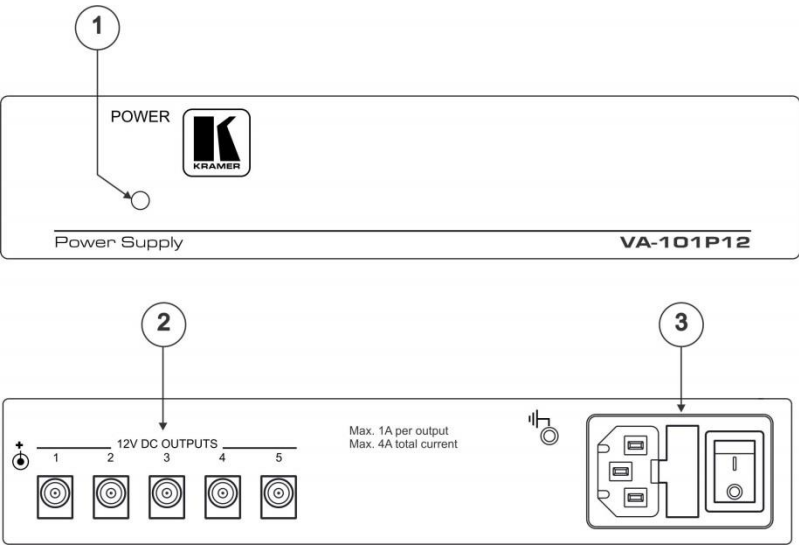
Figure 1: VA-101P12 5-Output 12V DC Power Supply
