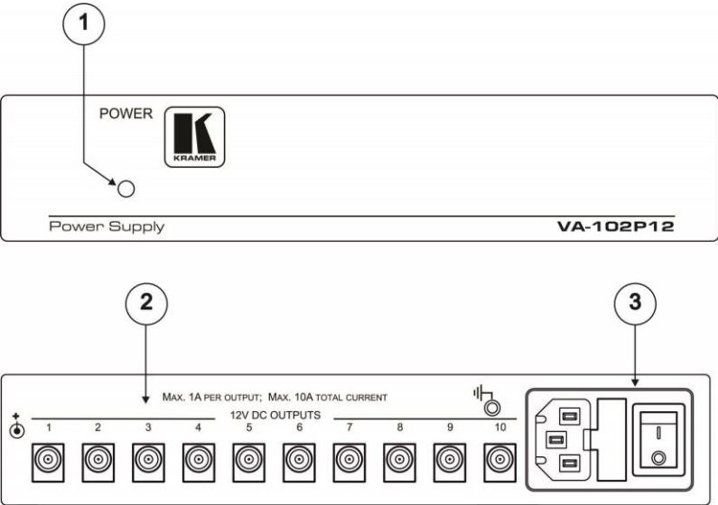
Figure 2: VA-102P12 10-Output 12V DC Power Supply
